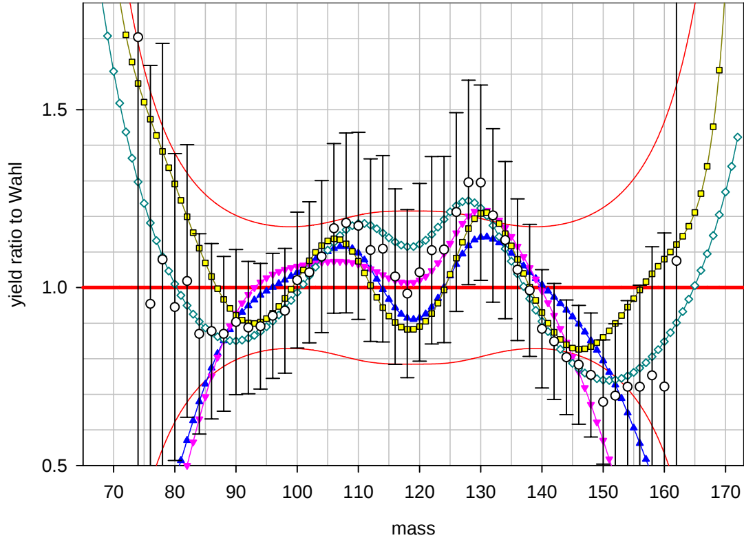
Benchmark A: ^{238}\text{U} around 28 MeV: pre neutron emission yield ratio to Wahl's systematics Lower graph: partial plot (very high and low values omitted); for legend see upper graph.
